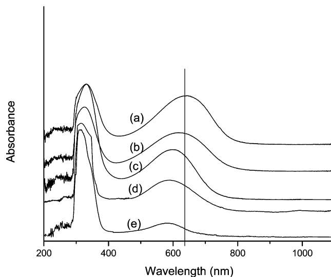
Figure 6. UV-vis spectra of (a) neutralized PANI, (b) neutralized poly((AP- g -PEO-750)- co -aniline) (1/2), (c) neutralized poly((AP- g -PEO-750)- co -aniline) (1/1), (d) neutralized poly((AP- g -PEO-750)- co -aniline) (3/1), and (e) neutralized poly((AP- g -PEO-750)- co -aniline) (6/1) (all in DMF).
