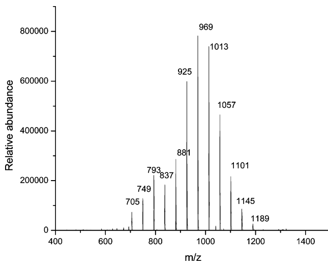
Figure 2. MS spectrum of AP-Boc- g -PEO-750.
