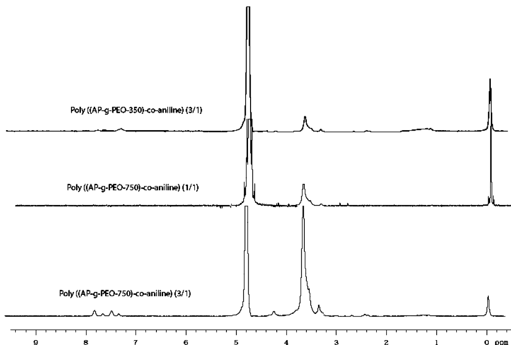
Figure 4. ^1\text{H} NMR spectra of copolymers in \text{D}_2\text{O} , 5 g/L: (a) poly((AP- g -PEO-750)- co -aniline) (3/1), (b) poly((AP- g -PEO-750)- co -aniline) (1/1), and (c) poly((AP- g -PEO-350)- co -aniline) (3/1).
