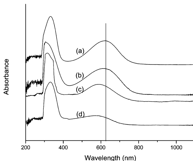
Figure 8. UV-vis spectra of (a) neutralized poly((AP- g -PEO-150)- co -aniline) (3/1), (b) neutralized poly((AP- g -PEO-350)- co -aniline) (3/1), (c) neutralized poly((AP- g -PEO-750)- co -aniline) (3/1), and (d) neutralized poly((AP- g -PEO-2000)- co -aniline) (3/1) (all in DMF).
