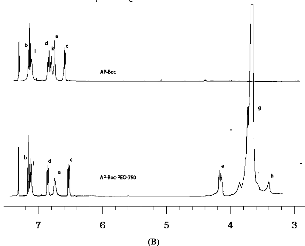
Figure 3. (A) ^1\text{H} NMR spectra of (a) 3-aminophenol, (b) AP-Boc, (c) AP-Boc- g -PEO-750, (d) AP- g -PEO-750, and (e) poly((AP- g -PEO)- co -aniline) (3/1) in \text{CDCl}_3 , 5 g/L. (B) Two expanded ^1\text{H} NMR spectra of (b) AP-Boc and (c) AP-Boc- g -PEO-750 in \text{CDCl}_3 , 5 g/L.
