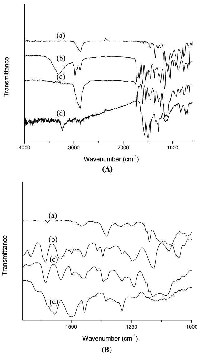
Figure 1. FTIR spectra of (a) PEO-750-Tos, (b) AP-Boc, (c) AP-Boc- g -PEO-750, and (d) poly(AP- g -PEO-750)- co -aniline (3/1).
