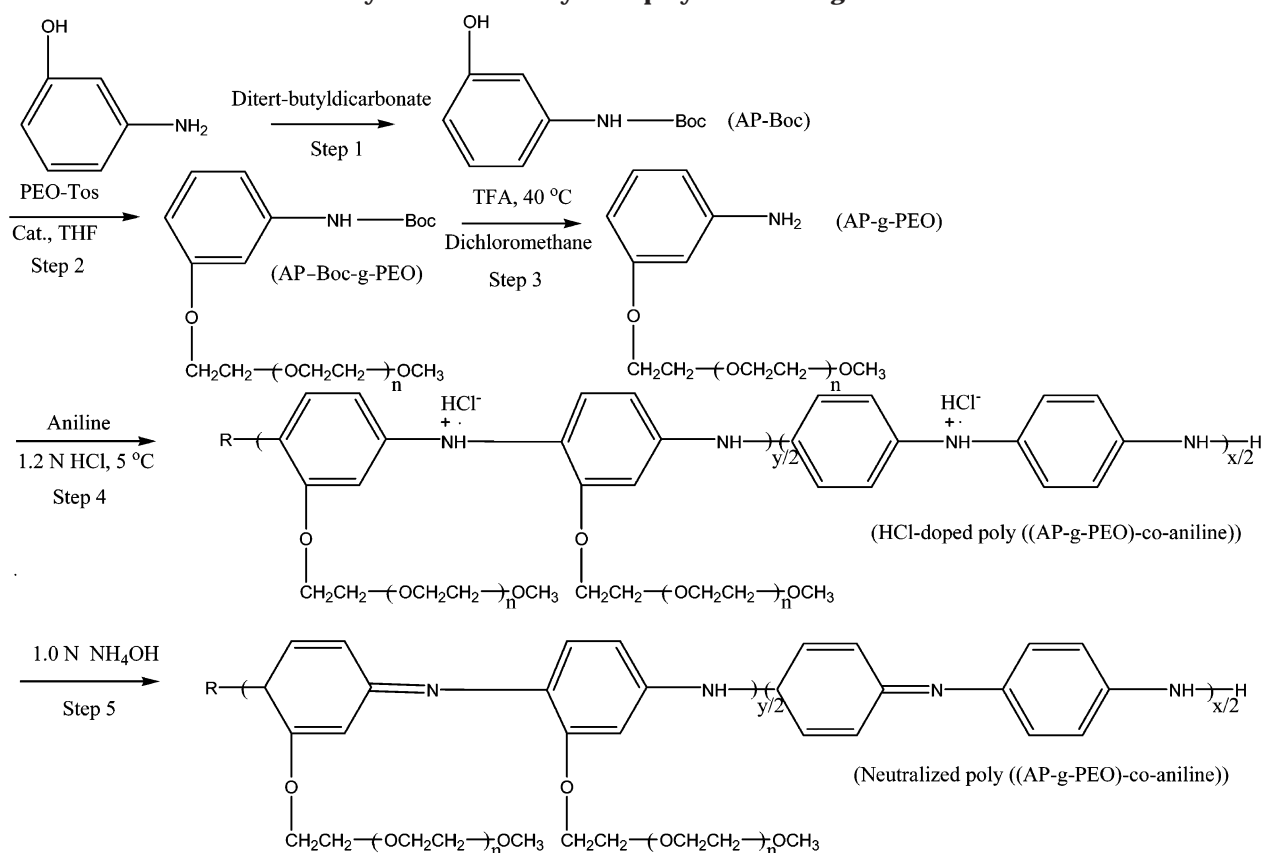
Scheme 1. Synthesis Pathway of Copolymers of AP- g -PEO and Aniline
