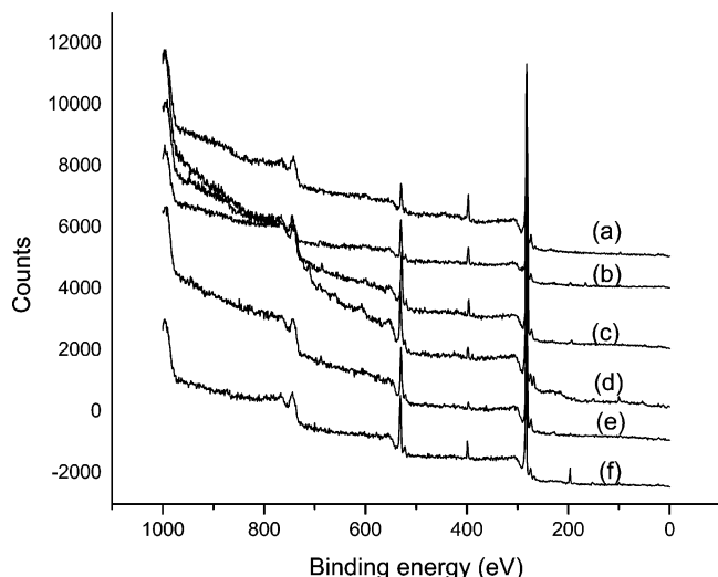
Figure 9. XPS spectra of copolymers: (a) neutralized poly( o -anisidine), (b) neutralized poly((AP- g -PEO-750)- co -aniline) (3/1), (c) neutralized poly((AP- g -PEO-750)- co -aniline) (1/1), (d) neutralized poly((AP- g -PEO-350)- co -aniline) (1/2), (e) neutralized poly(AP- g -PEO-750), and (f) HCl-doped poly((AP- g -PEO-750)- co -aniline) (3/1).
