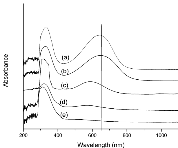
Figure 5. UV-vis spectra of (a) neutralized PANI, (b) neutralized poly( o -anisidine), (c) neutralized poly((AP- g -PEO-750)- co -aniline) (3/1), (d) neutralized poly(2-aminophenol), and (e) neutralized poly(AP- g -PEO-750) (all in DMF).
